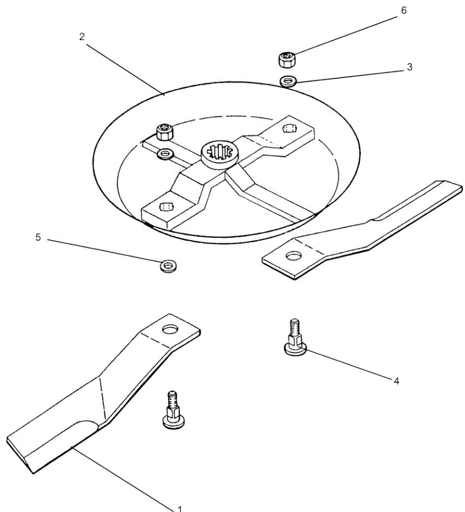
2 BLADE ASSY
