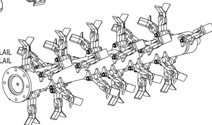
184.733S - 1.2M ROTOR (30 STATION) BOOT FLAIL
