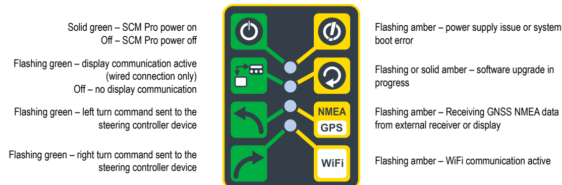
Figure 2: LED panel
