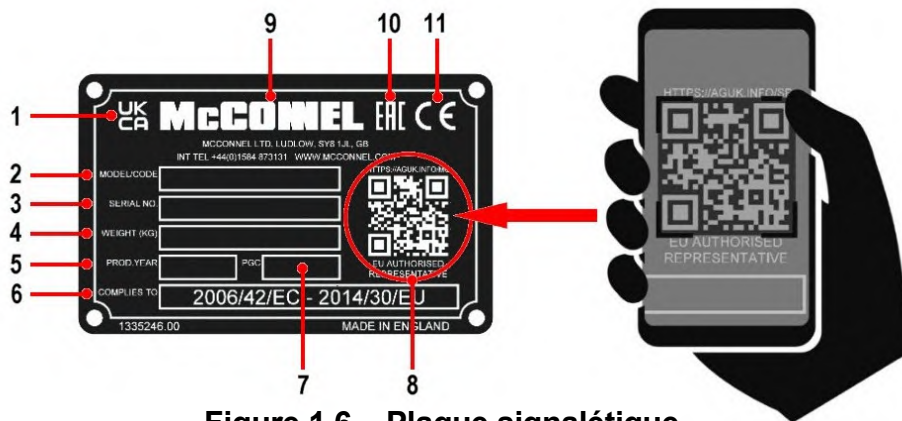
Figure 1.6 – Plaque signalétique
