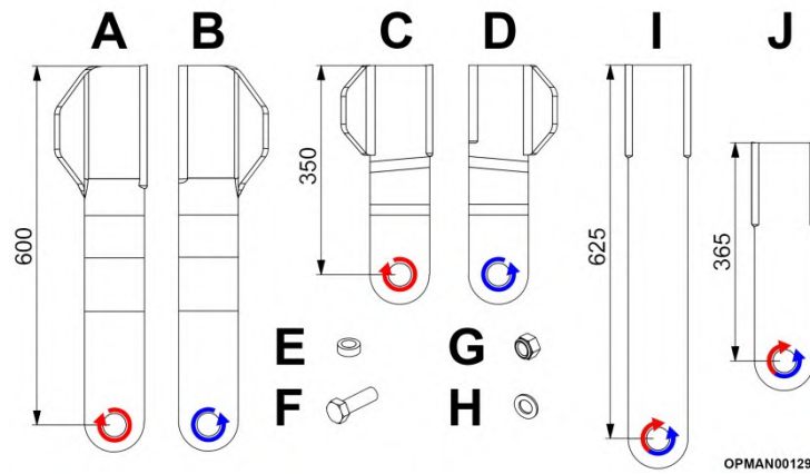
Figure 5.49 Composants des lames standard & lames Starcut
