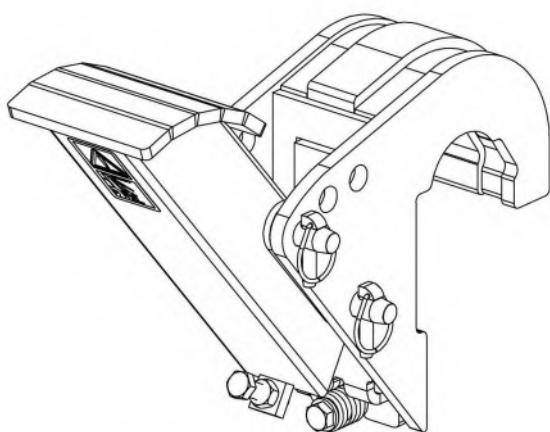
Transport Position
